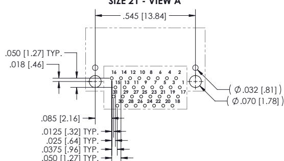
SIZE 31 - VIEW A
