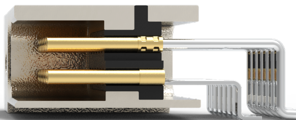
Socket with Crimped Round Surface-Mount Lead vs. Socket with Integral Tail Surface-Mount Lead
